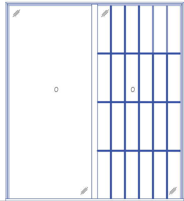
Direct Glazed Available up to \infty Panels 11'-6" x 6'-8"
